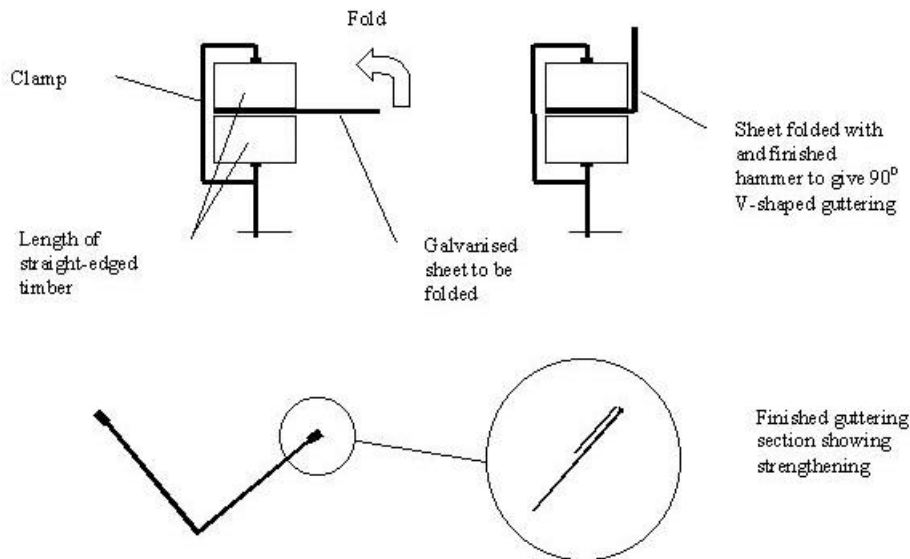
Figure 6: folding galvanised steel sheet to make V-shaped guttering
