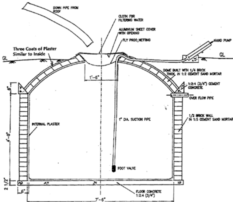
Figure 16: detail drawing of the Sri Lankan brick dome tank
