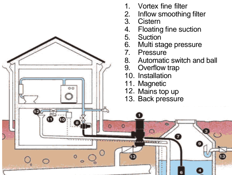
Figure 20: a typical European RWH system (Source: Construction Resources News, Winter 1997)
