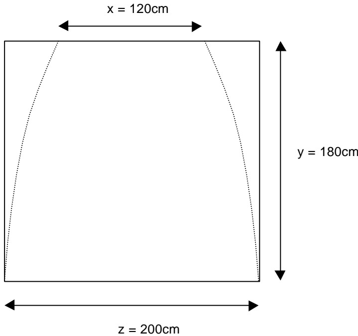
Figure 19: Dimensions for cutting sacking
