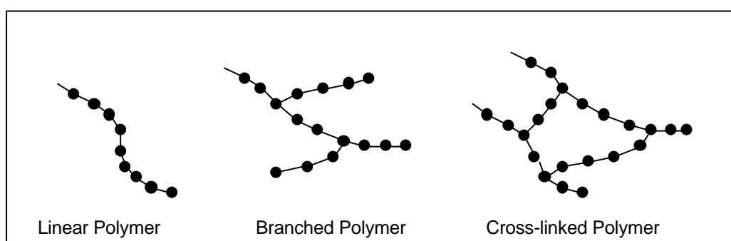
Figure 1: Polymer structures
